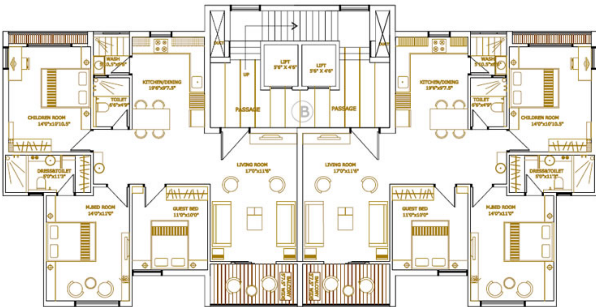
PROPOSED TYPICAL FLOOR PLAN FOR TOWER "B", SPRING'S RETREAT -2, VASNA-BHAILY ROAD, VADODARA.
